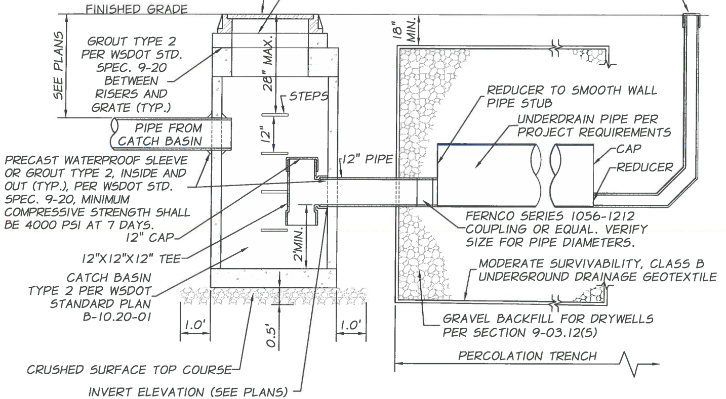
CROSS SECTION NTS
